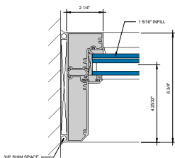
⑦ JAMB AT FIXED LITE S P = 1'-0"
