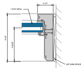
⑩ JAMB AT FIXED LITE 6\"/>
