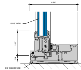
③ SILL AT SLIDING PANEL (UNDER 90 PSF) 6\"/>
