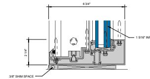
⑥ SILL AT FIXED LITE (UNDER 90 PSF) 6\"/>
