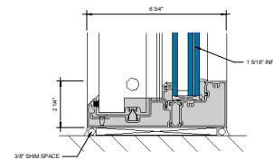
⑥ SILL AT FIXED LITE (UNDER 90 PSF) 0" = 1'-0"
