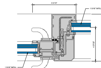
⑨ LOCK STILE MULLION S P = 1'-0"
