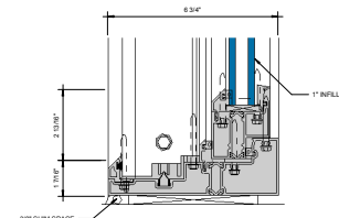
⑧ SILL AT FIXED LITE (UNDER 90 PSF) 6\" = 1'-0"
