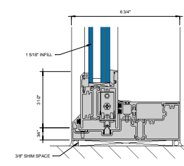
③ SILL AT SLIDING PANEL (UNDER 90 PSF) D" = 1'-0"
