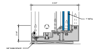
⑧ SILL AT FIXED LITE (UNDER 90 PSF) 6\"/>
