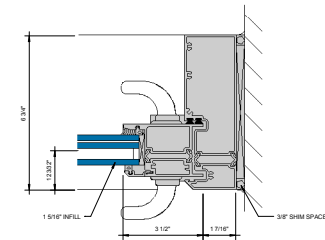
⑨ JAMB AT SLIDING PANEL 6\"/>
