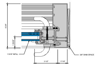
⑩ JAMB AT SLIDING PANEL 6\"/>
