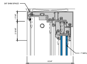
⑥ HEAD AT FIXED LITE 6\"/>
