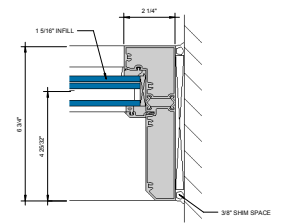
⑩ JAMB AT FIXED LITE S P = 1'-0"
