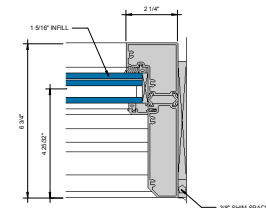
⑨ JAMB AT FIXED PANEL 6\"/>
