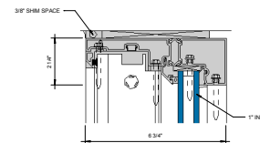
⑦ HEAD AT FIXED LITE 6\"/>
