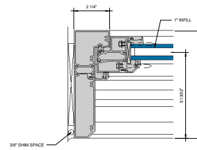
⑪ JAMB AT FIXED LITE 6\"/>
