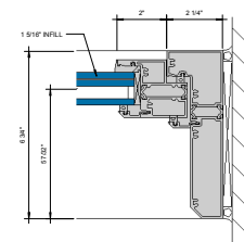
⑩ JAMB AT FIXED LITE 6" = 1'-0"
