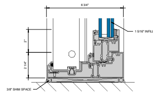
⑥ SILL AT FIXED LITE (UNDER 90 PSF) 6\"/>
