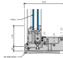
③ SILL AT SLIDING PANEL (UNDER 90 PSF) 6\"/>
