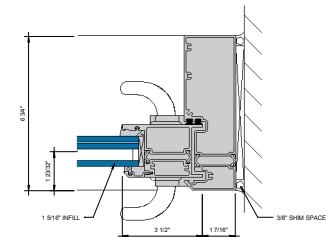
⑨ JAMB AT SLIDING PANEL 6" = 1'-0"
