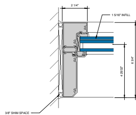
⑦ JAMB AT FIXED PANEL 6\" = 1'-0"
