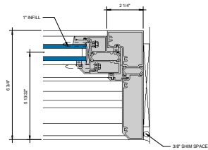
② JAMB AT FIXED LITE 6\" = 1'-0\"
