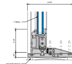
④ LOW RISE SILL AT SLIDING PANEL (UNDER 90 PSF) 6\" = 1'-0"
