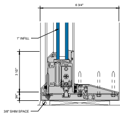
⑤ LOW RISE SILL AT SLIDING PANEL (UNDER 90 PSF) 6\"/>
