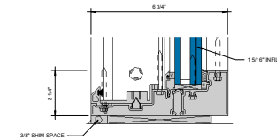
⑥ SILL AT FIXED LITE (UNDER 90 PSF) 6\"/>
