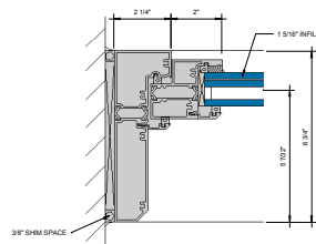
⑦ JAMB AT FIXED LITE Ø" = 1'-0"
