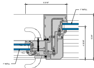
① LOCK STILE MULLION 6" = 1'-0"
