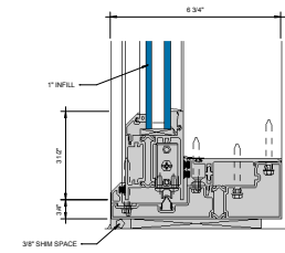
④ SILL AT SLIDING PANEL (UNDER 90 PSF) 6\"/>
