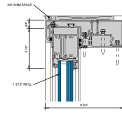
② HEAD AT SLIDING PANEL (UNDER 90 PSF) 6\"/>
