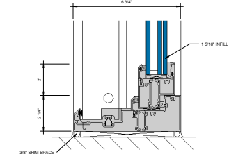
⑥ SILL AT FIXED LITE (UNDER 90 PSF) 6" = 1'-0"
