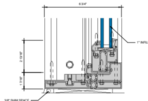
⑨ LOW RISE SILL AT FIXED LITE (UNDER 90 PSF) 6\"/>
