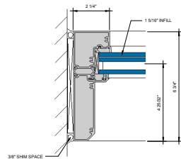
⑦ JAMB AT FIXED LITE 0" = 1'-0"
