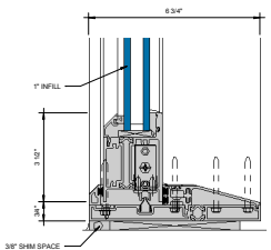
LOW RISE SILL AT SLIDING PANEL (UNDER 90 PSF) ⑤ 6\"/>
