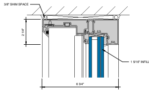
④ HEAD AT FIXED LITE 6\"/>
