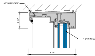
④ HEAD AT FIXED LITE 6\"/>
