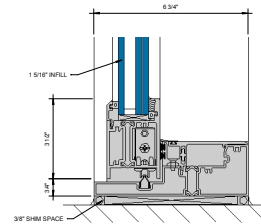
② SILL AT SLIDING PANEL (UNDER 90 PSF) Ø" = 1'-0"
