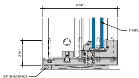
⑨ LOW RISE SILL AT FIXED LITE (UNDER 90 PSF) 6\"/>
