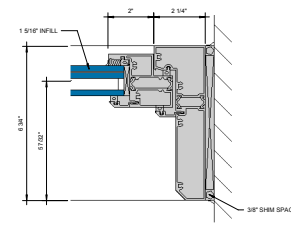
⑪ JAMB AT FIXED LITE 6\"/>
