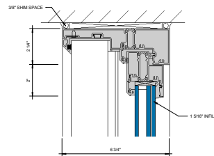
④ HEAD AT FIXED LITE D' = 1'-0"
