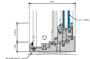
⑧ SILL AT FIXED LITE (UNDER 90 PSF) 6\"/>
