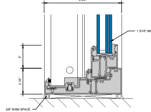
⑥ SILL AT FIXED LITE (UNDER 80 PSF) D" = 1'-0"
