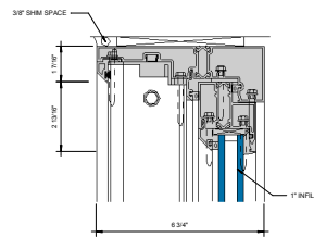
⑥ HEAD AT FIXED LITE 6\" = 1'-0"
