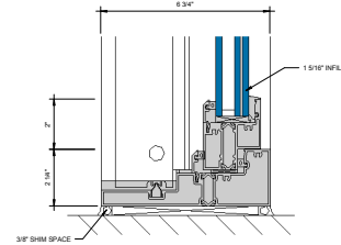
⑤ SILL AT FIXED LITE (UNDER 80 PSF) D" = 1'-0"
