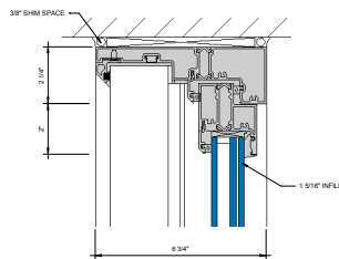
④ HEAD AT FIXED LITE D" = 1'-0"
