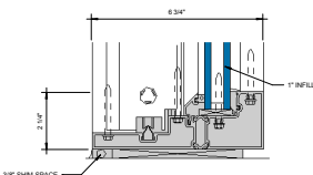
⑨ SILL AT FIXED LITE (UNDER 90 PSF) 6\"/>
