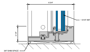
⑤ SILL AT FIXED LITE (UNDER 90 PSF) 6\"/>
