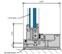
③ SILL AT SLIDING PANEL (UNDER 90 PSF) Ø" = 1'-0"
