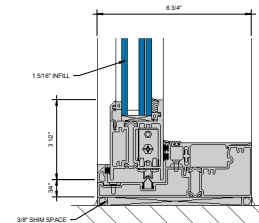
③ SILL AT SLIDING PANEL (UNDER 80 PSF) D = 1'-0"
