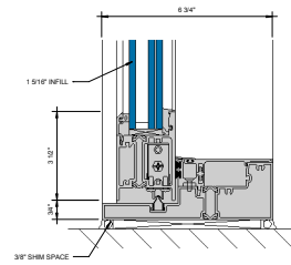
② SILL AT SLIDING PANEL (UNDER 90 PSF) 0" = 1'-0"
