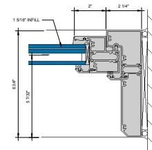
⑨ JAMB AT FIXED LITE D" = 1'-0"
