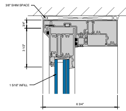
① HEAD AT SLIDING PANEL S 1 = 1'-0"
