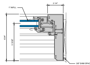
② JAMB AT FIXED LITE 0\"/>
