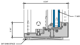
⑦ SILL AT FIXED LITE (UNDER 90 PSF) 6\"/>
