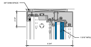
④ HEAD AT FIXED LITE 6\"/>
