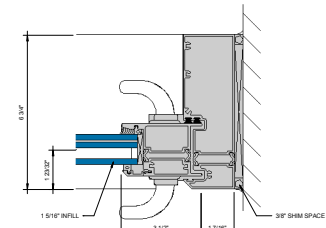
⑩ JAMB AT SLIDING PANEL 0\"/>
