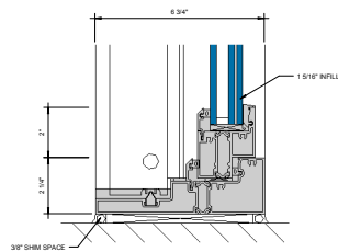
⑤ SILL AT FIXED LITE (UNDER 90 PSF) S 1 = 1'-0"
