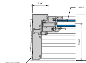
⑪ JAMB AT FIXED LITE 6\"/>
