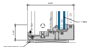
⑩ SILL AT FIXED LITE (UNDER 90 PSF) 6\"/>
