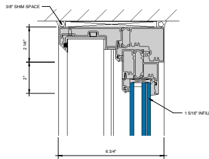
④ HEAD AT FIXED LITE 6" = 1'-0"
