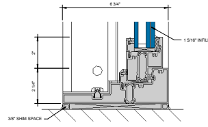
⑤ SILL AT FIXED LITE (UNDER 90 PSF) D = 1'-0"
