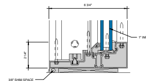
⑦ SILL AT FIXED LITE (UNDER 90 PSF) 6\"/>
