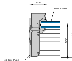
⑪ JAMB AT FIXED LITE 6\"/>
