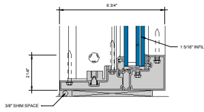
⑤ SILL AT FIXED LITE (UNDER 90 PSF) 6\"/>
