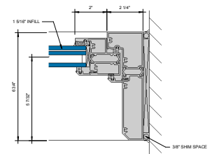
⑩ JAMB AT FIXED LITE D = 1'-0"
