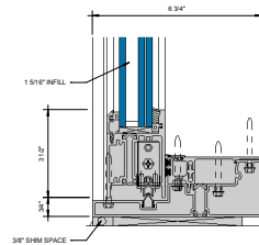
② SILL AT SLIDING PANEL (UNDER 90 PSF) 6\"/>
