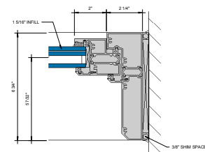
⑩ JAMB AT FIXED LITE D = 1'-0"
