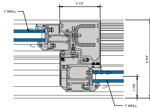
① INTERLOCK 6" = 1'-0"
