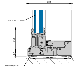
③ SILL AT SLIDING PANEL (UNDER 90 PSF) 6\"/>
