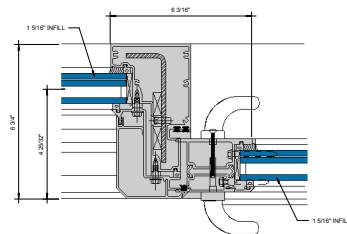
⑧ LOCK STILE MULLION 6\"/>
