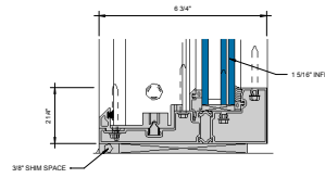
⑥ SILL AT FIXED LITE (UNDER 90 PSF) 6\"/>
