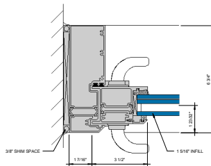
⑦ JAMB AT SLIDING PANEL 0\"/>
