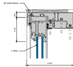
HEAD AT SLIDING PANEL (UNDER 90 PSF) ② 6\"/>
