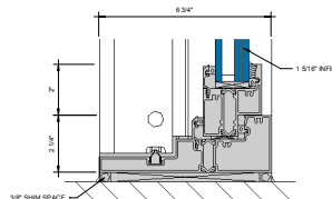
⑤ SILL AT FIXED LITE (UNDER 90 PSF) 0\"/>
