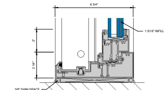
⑥ SILL AT FIXED LITE (UNDER 90 PSF) 0\"/>
