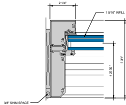
⑦ JAMB AT FIXED PANEL 6\"/>
