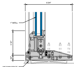
⑤ LOW RISE SILL AT SLIDING PANEL (UNDER 90 PSF) 6\" = 1'-0"
