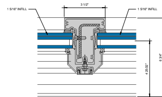
⑧ FIXED MULLION 6\"/>
