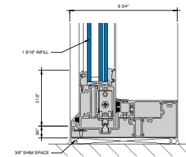
③ SILL AT SLIDING PANEL (UNDER 90 PSF) 6\" = 1'-0"
