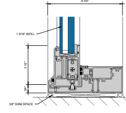
③ SILL AT SLIDING PANEL (UNDER 80 PSF) D" = 1'-0"
