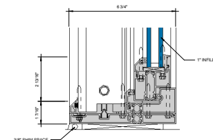
⑩ LOW RISE SILL AT FIXED LITE (UNDER 90 PSF) 6\" = 1'-0"
