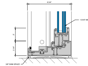
⑥ SILL AT FIXED LITE (UNDER 90 PSF) D' = 1'-0"
