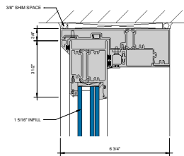
① HEAD AT SLIDING PANEL S P = 1'-0"
