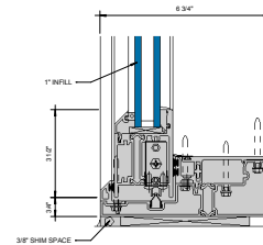
③ SILL AT SLIDING PANEL (UNDER 90 PSF) 6\"/>
