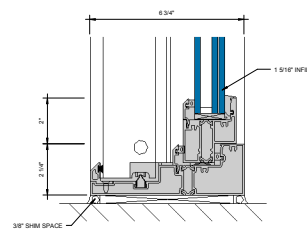
⑥ SILL AT FIXED LITE (UNDER 90 PSF) S 1 = 1'-0"
