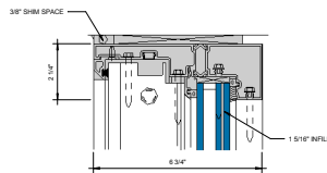
⑤ HEAD AT FIXED LITE 6\"/>
