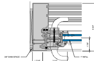
⑪ LOCK JAMB AT SLIDING PANEL 6\"/>
