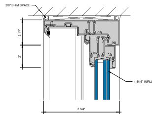
④ HEAD AT FIXED LITE 6\"/>
