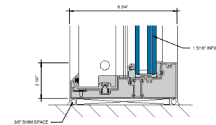
⑥ SILL AT FIXED LITE (UNDER 90 PSF) 6\" = 1'-0"
