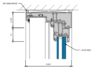
④ HEAD AT FIXED LITE 6" = 1'-0"
