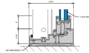
⑥ SILL AT FIXED LITE (UNDER 80 PSF) D = 1'-0"
