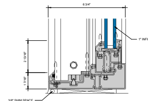
⑧ SILL AT FIXED LITE (UNDER 90 PSF) 6\"/>
