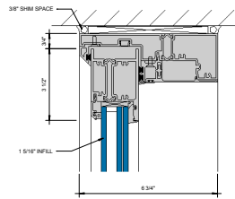
① HEAD AT SLIDING PANEL 0" = 1'-0"
