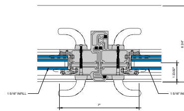
⑪ MEETING STILE 6\"/>
