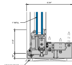
③ SILL AT SLIDING PANEL (UNDER 90 PSF) 6\" = 1'-0"
