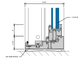
⑥ SILL AT FIXED LITE (UNDER 90 PSF) 6\"/>
