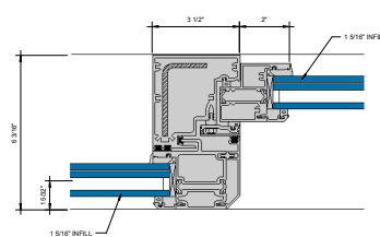
⑧ INTERLOCKS D" = 1'-0"
