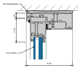
① HEAD AT SLIDING PANEL Ø" = 1'-0"
