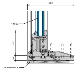
⑤ LOW RISE SILL AT SLIDING PANEL (UNDER 90 PSF) 6\"/>
