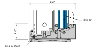
⑥ SILL AT FIXED LITE (UNDER 90 PSF) 0\"/>
