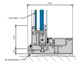
③ SILL AT SLIDING PANEL (UNDER 90 PSF) S P = 1'-0"
