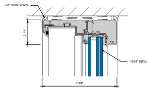
④ HEAD AT FIXED LITE 6\"/>
