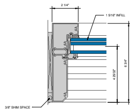
⑨ JAMB AT FIXED PANEL 6\"/>
