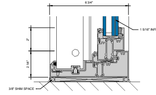
⑥ SILL AT FIXED LITE (UNDER 90 PSF) D = 1'-0"
