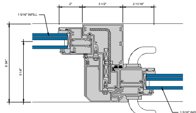
⑧ LOCK STILE MULLION 6" = 1'-0"
