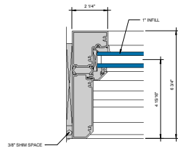
① JAMB AT FIXED LITE 6" = 1'-0"
