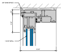
① HEAD AT SLIDING PANEL 6\"/>
