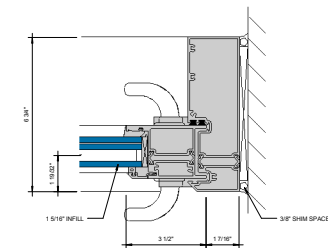
⑨ JAMB AT SLIDING PANEL 6\" = 1'-0"
