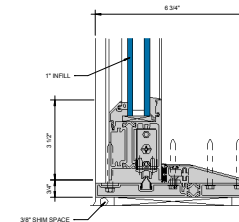
④ LOW RISE SILL AT SLIDING PANEL (UNDER 90 PSF) 6\"/>
