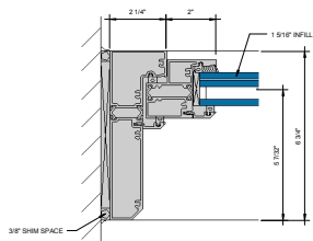
⑦ JAMB AT FIXED LITE D = 1'-0"
