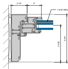
⑦ JAMB AT FIXED LITE 6" = 1'-0"
