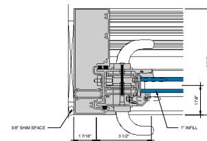
⑪ JAMB AT SLIDING PANEL 6\"/>
