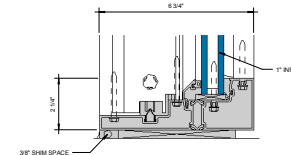
⑦ SILL AT FIXED LITE (UNDER 90 PSF) 6\"/>
