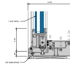
④ SILL AT SLIDING PANEL (UNDER 90 PSF) 6\"/>
