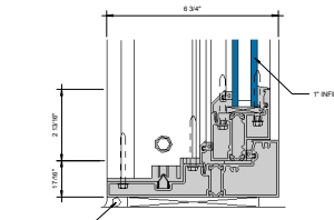
⑦ SILL AT FIXED LITE (UNDER 90 PSF) 6\" = 1'-0"
