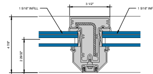
⑨ FIXED MULLION 6\"/>
