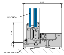
③ SILL AT SLIDING PANEL (UNDER 90 PSF) 6" = 1'-0"
