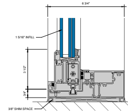
③ SILL AT SLIDING PANEL (UNDER 90 PSF) 0\"/>
