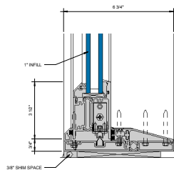
⑤ LOW RISE SILL AT SLIDING PANEL (UNDER 90 PSF) 6\"/>
