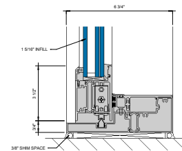
② SILL AT SLIDING PANEL (UNDER 90 PSF) 6\"/>
