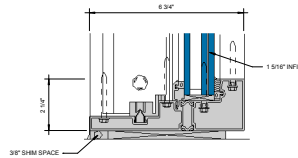
⑤ SILL AT FIXED LITE (UNDER 90 PSF) 6\"/>
