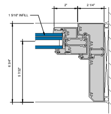
⑪ JAMB AT FIXED LITE S 1 = 1'-0"
