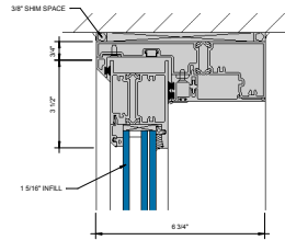
① HEAD AT SLIDING PANEL D = 1'-0"
