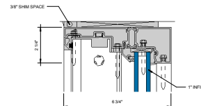
⑥ HEAD AT FIXED LITE 6\"/>
