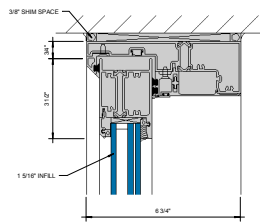
① HEAD AT SLIDING PANEL 6\"/>
