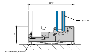
⑥ SILL AT FIXED LITE (UNDER 90 PSF) S P = 1'-0"
