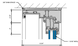
④ HEAD AT FIXED LITE Ø" = 1'-0"
