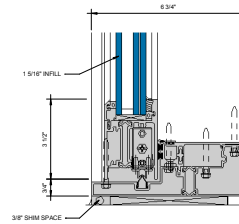
② SILL AT SLIDING PANEL (UNDER 90 PSF) 6\"/>
