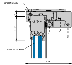
① HEAD AT SLIDING PANEL 6\"/>
