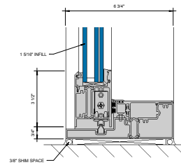
② SILL AT SLIDING PANEL (UNDER 90 PSF) D" = 1'-0"
