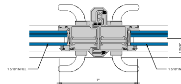
⑨ MEETING STILE 0" = 1'-0"
