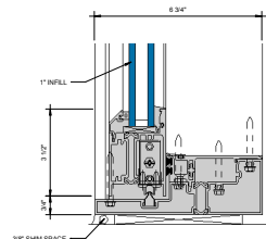
② SILL AT SLIDING PANEL (UNDER 90 PSF) 6\" = 1'-0"
