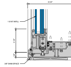
③ SILL AT SLIDING PANEL (UNDER 90 PSF) 6\"/>
