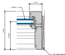
⑤ JAMB AT FIXED LITE 6" = 1'-0"
