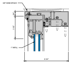
① HEAD AT SLIDING PANEL 6\" = 1'-0"
