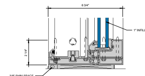
LOW RISE SILL AT FIXED LITE (UNDER 90 PSF) ⑫ 6\"/>
