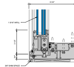
③ SILL AT SLIDING PANEL (UNDER 90 PSF) 0\"/>
