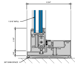
② SILL AT SLIDING PANEL (UNDER 90 PSF) 6\"/>
