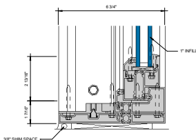
⑨ LOW RISE SILL AT FIXED LITE (UNDER 90 PSF) 6\"/>
