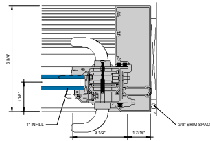
② JAMB AT SLIDING PANEL 6" = 1'-0"
