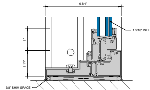
⑤ SILL AT FIXED LITE (UNDER 90 PSF) Ø" = 1'-0"
