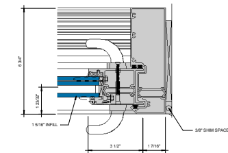
⑨ JAMB AT SLIDING PANEL 6\"/>
