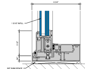
③ SILL AT SLIDING PANEL (UNDER 90 PSF) 6" = 1'-0"
