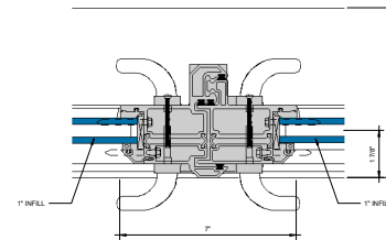
③ MEETING STILE 6" = 1'-0"
