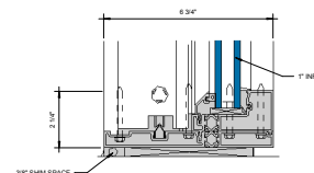
LOW RISE SILL AT FIXED LITE (UNDER 90 PSF) ⑪ 6\"/>
