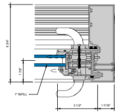
② LOCK JAMB AT SLIDING PANEL 8\"/>
