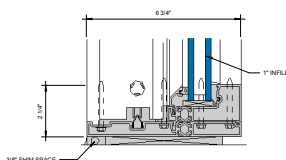
⑨ LOW RISE SILL AT FIXED LITE (UNDER 90 PSF) 6\"/>
