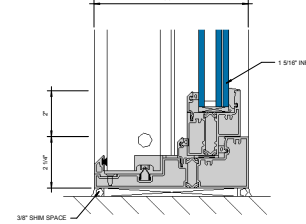
⑥ SILL AT FIXED LITE (UNDER 90 PSF) 6" = 1'-0"
