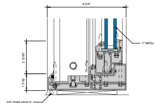
⑩ LOW RISE SILL AT FIXED LITE (UNDER 90 PSF) 6\"/>
