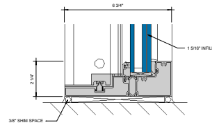
⑤ SILL AT FIXED LITE (UNDER 90 PSF) 6\"/>
