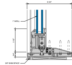
LOW RISE SILL AT SLIDING PANEL (UNDER 90 PSF) ④ 6\"/>
