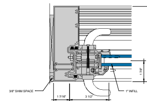
⑪ LOCK JAMB AT SLIDING PANEL 6\"/>
