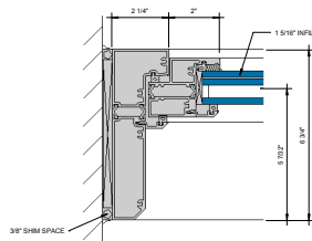
⑦ JAMB AT FIXED LITE 0\"/>
