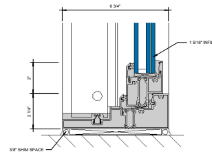
⑤ SILL AT FIXED LITE (UNDER 90 PSF) D' = 1'-0"
