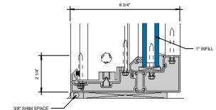
⑧ SILL AT FIXED LITE (UNDER 90 PSF) 6\"/>
