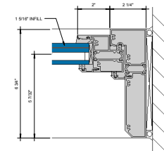
⑩ JAMB AT FIXED LITE D" = 1'-0"
