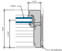
② JAMB AT FIXED LITE 6\" = 1'-0"
