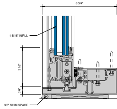
② SILL AT SLIDING PANEL (UNDER 90 PSF) 6\"/>
