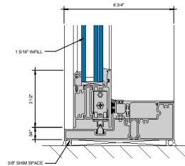
② SILL AT SLIDING PANEL (UNDER 90 PSF) 6\"/>
