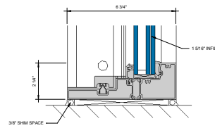
⑤ SILL AT FIXED LITE (UNDER 90 PSF) S P = 1'-0"
