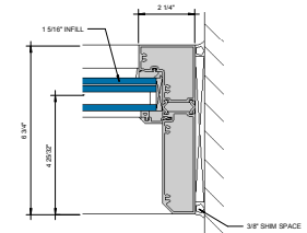
⑩ JAMB AT FIXED PANEL 6\"/>
