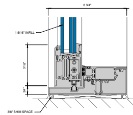
② SILL AT SLIDING PANEL UNDER 90 PSF S 1 = 1'-0"
