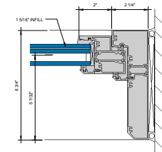
⑩ JAMB AT FIXED LITE D' = 1'-0"
