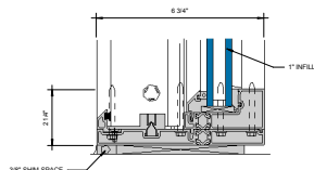
LOW RISE SILL AT FIXED LITE (UNDER 90 PSF) ⑩ 6\"/>
