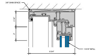
④ HEAD AT FIXED LITE 6\"/>
