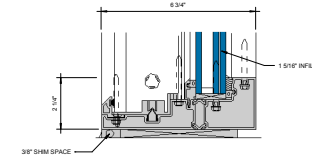
⑧ SILL AT FIXED LITE (UNDER 90 PSF) 6\"/>
