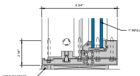
LOW RISE SILL AT FIXED LITE (UNDER 90 PSF) ⑨ 6\"/>
