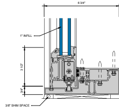
② SILL AT SLIDING PANEL (UNDER 90 PSF) 6\"/>
