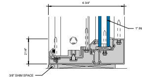
⑧ SILL AT FIXED LITE (UNDER 90 PSF) 6\"/>
