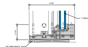
⑨ LOW RISE SILL AT FIXED LITE (UNDER 90 PSF) 6\"/>
