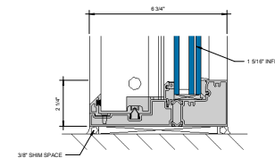
⑥ SILL AT FIXED LITE (UNDER 90 PSF) 6\"/>
