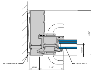
⑦ JAMB AT SLIDING PANEL D' = 1'-0"
