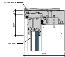
① HEAD AT SLIDING PANEL 0\"/>
