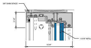
④ HEAD AT FIXED LITE 0\"/>
