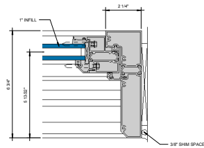
⑤ JAMB AT FIXED LITE Ø = 1"0"
