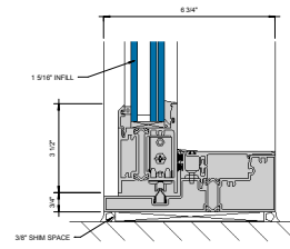
② SILL AT SLIDING PANEL (UNDER 90 PSF) 6" = 1'-0"
