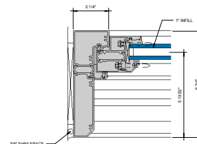
⑪ JAMB AT FIXED LITE 6\" = 1'-0"
