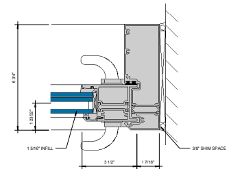
⑩ JAMB AT SLIDING PANEL 6\"/>
