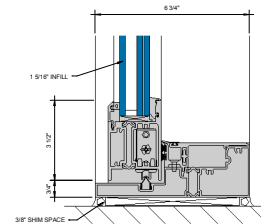
② SILL AT SLIDING PANEL (UNDER 90 PSF) D' = 1'-0"
