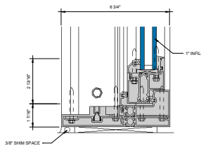
⑨ LOW RISE SILL AT FIXED LITE (UNDER 90 PSF) 6\"/>
