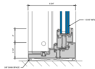
⑤ SILL AT FIXED LITE (UNDER 90 PSF) 6\"/>
