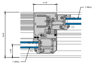
① INTERLOCK 6\" = 1'-0\"
