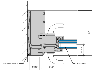
⑦ JAMB AT SLIDING PANEL D = 1'-0"
