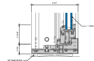
⑨ LOW RISE SILL AT FIXED LITE (UNDER 90 PSF) 6\" = 1'-0"
