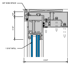
① HEAD AT SLIDING PANEL 6\"/>
