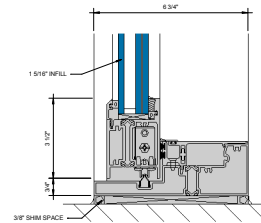
② SILL AT SLIDING PANEL (UNDER 90 PSF) 0\"/>
