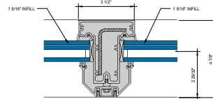
⑧ FIXED MULLION 6\"/>
