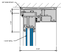
① HEAD AT SLIDING PANEL 6\"/>
