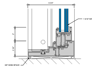
⑤ SILL AT FIXED LITE (UNDER 90 PSF) 6" = 1'-0"
