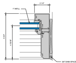
② JAMB AT FIXED LITE 6" = 1'-0"
