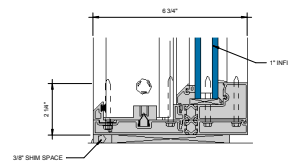
⑩ LOW RISE SILL AT FIXED LITE (UNDER 90 PSF) 6\"/>
