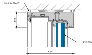
④ HEAD AT FIXED LITE 0" = 1'-0"
