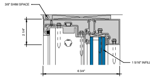
④ HEAD AT FIXED LITE 6\"/>
