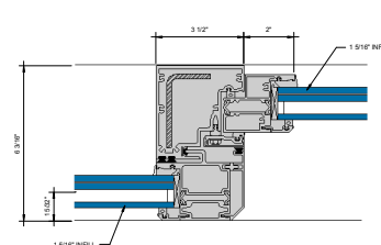
⑨ INTERLOCKS 6" = 1'-0"
