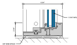
⑤ SILL AT FIXED LITE (UNDER 90 PSF) 0" = 1'-0"
