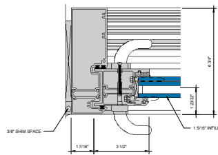
⑦ JAMB AT SLIDING PANEL 6\"/>
