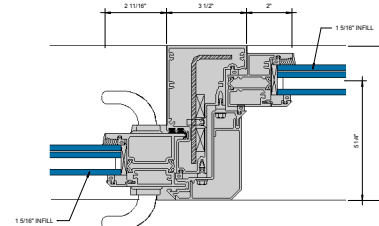
⑨ LOCK STILE MULLION Ø" = 1'-0"
