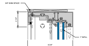
⑧ HEAD AT FIXED LITE (UNDER 90 PSF) 6\"/>
