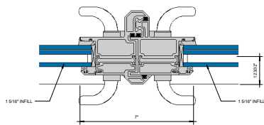
⑨ MEETING STILE S 1 = 1'-0"
