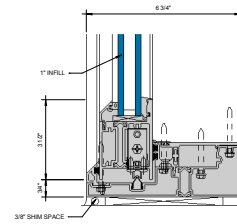
③ SILL AT SLIDING PANEL (UNDER 90 PSF) 6\"/>
