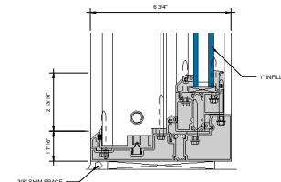
⑧ SILL AT FIXED LITE (UNDER 90 PSF) 6\"/>
