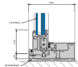
③ SILL AT SLIDING PANEL (UNDER 90 PSF) D = 1'-0"
