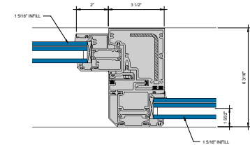
⑧ INTERLOCKS S 1 = 1'-0"
