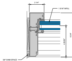
⑦ JAMB AT FIXED PANEL 0\"/>
