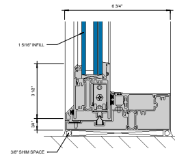
③ SILL AT SLIDING PANEL (UNDER 90 PSF) 0" = 1'-0"
