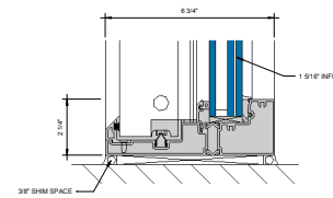
⑥ SILL AT FIXED LITE (UNDER 90 PSF) 6\"/>
