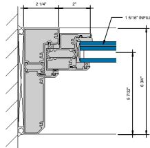
⑦ JAMB AT FIXED LITE D" = 1'-0"
