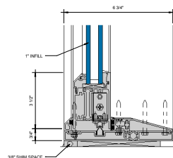
LOW RISE SILL AT SLIDING PANEL (UNDER 90 PSF) ⑥ 6\"/>
