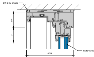
④ HEAD AT FIXED LITE D = 1'-0"
