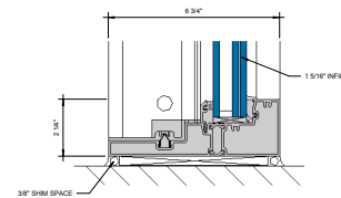
⑤ SILL AT FIXED LITE (UNDER 90 PSF) 6\" = 1'-0"
