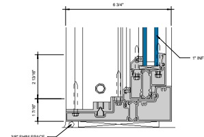
⑦ SILL AT FIXED LITE (UNDER 90 PSF) 6\"/>
