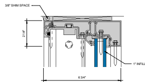
⑥ HEAD AT FIXED LITE 6\"/>
