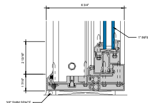
⑩ LOW RISE SILL AT FIXED LITE (UNDER 90 PSF) 6\"/>
