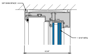
④ HEAD AT FIXED LITE S P = 1'-0"
