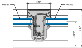
① FIXED MULLION 6" = 1'-0"
