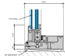
③ SILL AT SLIDING PANEL (UNDER 90 PSF) 6\"/>
