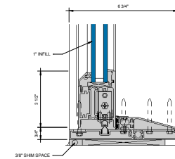
④ LOW RISE SILL AT SLIDING PANEL (UNDER 90 PSF) 6\"/>
