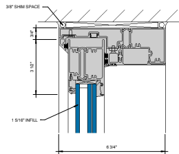
① HEAD AT SLIDING PANEL 6" = 1'-0"
