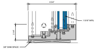
⑤ SILL AT FIXED LITE (UNDER 90 PSF) 0\"/>
