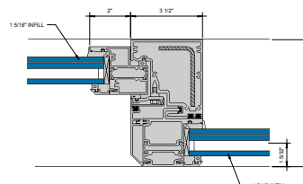
⑧ INTERLOCK 6" = 1'-0"
