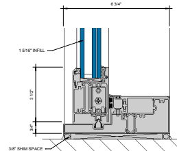
② SILL AT SLIDING PANEL (UNDER 90 PSF) 6\"/>
