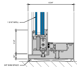
② SILL AT SLIDING PANEL (UNDER 90 PSF) 6\" = 1'-0"
