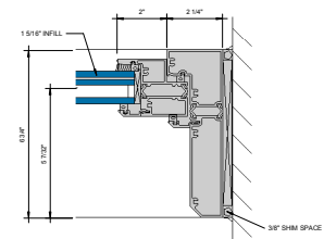
⑩ JAMB AT FIXED LITE Ø" = 1'-0"
