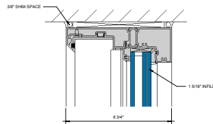
④ HEAD AT FIXED LITE 6\" = 1'-0"
