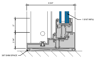
⑤ SILL AT FIXED LITE (UNDER 90 PSF) 6\"/>
