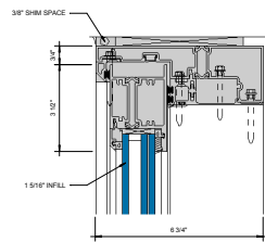
① HEAD AT SLIDING PANEL 6\"/>
