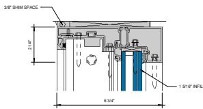
④ HEAD AT FIXED LITE 6\"/>
