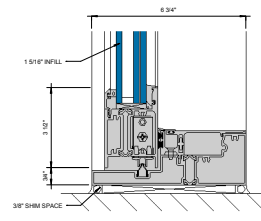
② SILL AT SLIDING PANEL (UNDER 90 PSF) S P = 1'-0"
