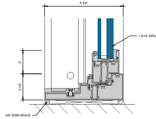
⑤ SILL AT FIXED LITE (UNDER 90 PSF) D" = 1'-0"
