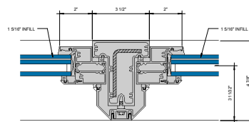
⑧ FIXED MULLION 6\"/>
