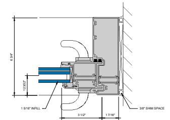
⑩ JAMB AT SLIDING PANEL 6\"/>
