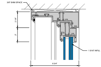
④ HEAD AT FIXED LITE S 1 = 1'-0"
