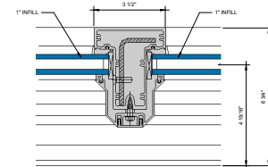
⑫ FIXED MULLION 6\"/>
