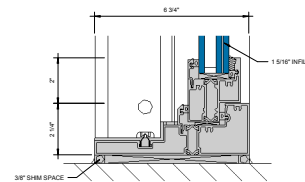
⑤ SILL AT FIXED LITE (UNDER 90 PSF) 0\"/>
