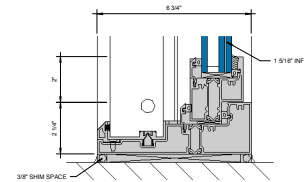
⑥ SILL AT FIXED LITE (UNDER 90 PSF) Ø" = 1'-0"
