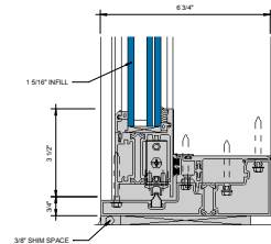
② SILL AT SLIDING PANEL (UNDER 90 PSF) 0\"/>
