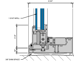
③ SILL AT SLIDING PANEL UNDER 90 PSF S 1 = 1'-0"
