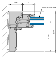
⑦ JAMB AT FIXED LITE 6" = 1'-0"
