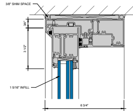
① HEAD AT SLIDING PANEL 0\"/>
