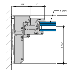
⑦ JAMB AT FIXED LITE S 1 = 1'-0"
