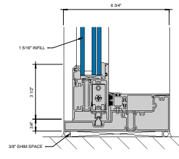
② SILL AT SLIDING PANEL (UNDER 80 PSF) D" = 1'-0"
