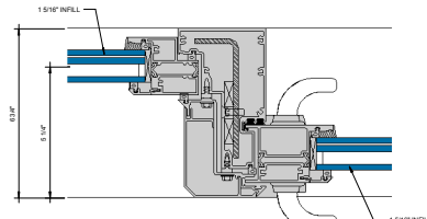
⑧ LOCK STILE MULLION D = 1'-0"
