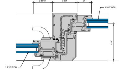
⑨ LOCK STILE MULLION D" = 1'-0"
