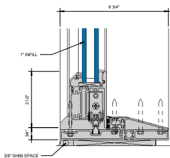
LOW RISE SILL AT SLIDING PANEL (UNDER 90 PSF) ⑤ 6\"/>
